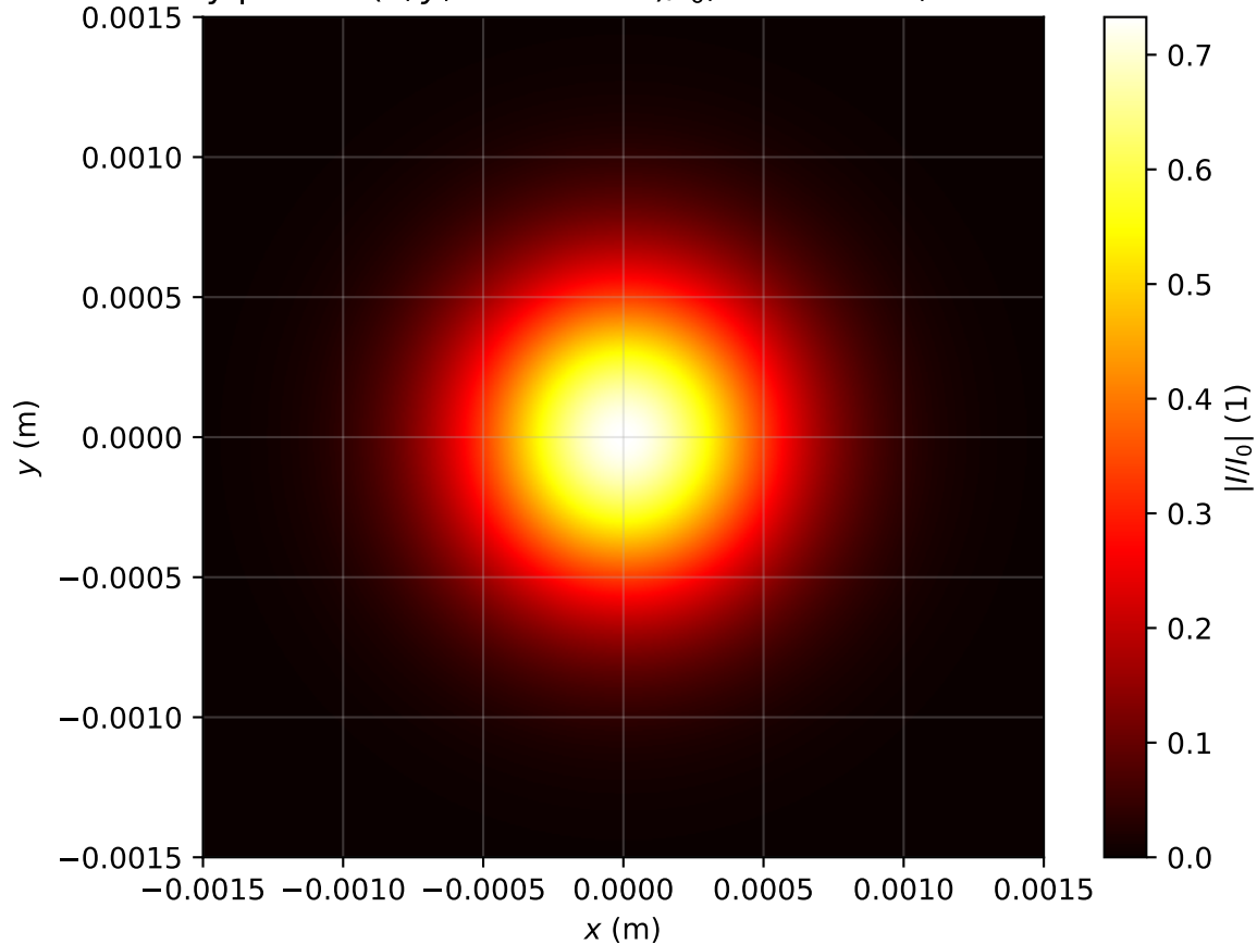
Intensity profile I(x, y, z = 1.513m)/I_0 , \text{Pin}=0.2\text{Pcr} , artificial time
